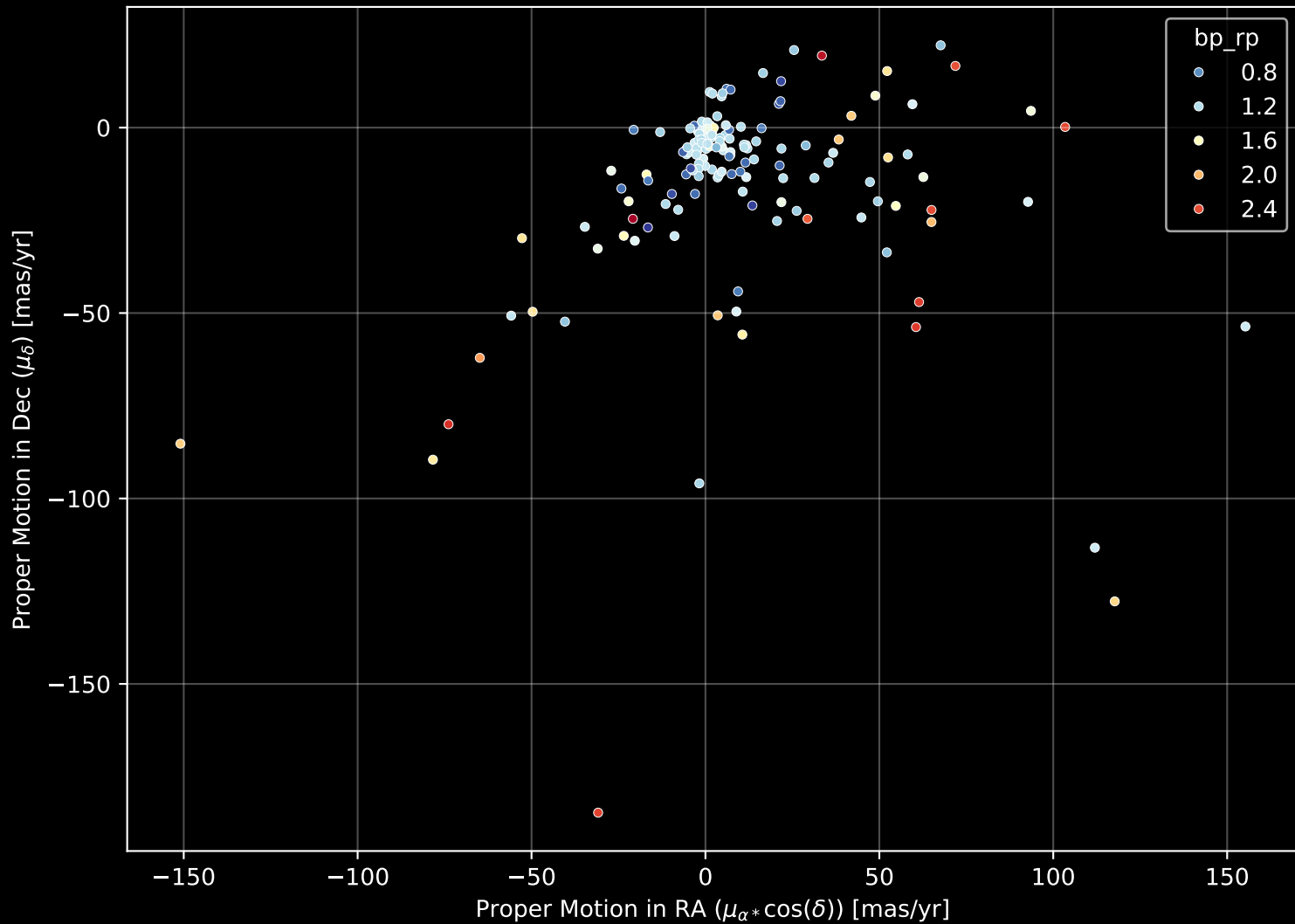
APOGEE DR17 Field: [120-45] Proper Motion Diagram (n= 159)
