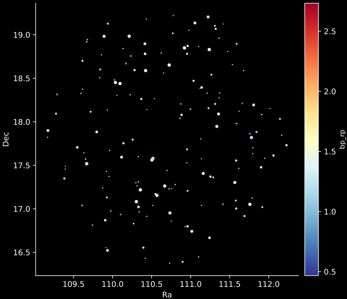
APOGEE DR17 Field: [120-45] Stars: 159
