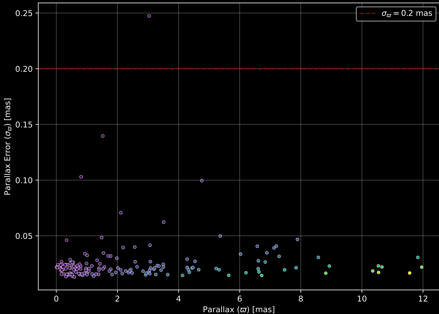
APOGEE DR17 Field: [120-45] Parallax Quality (n= 159)
