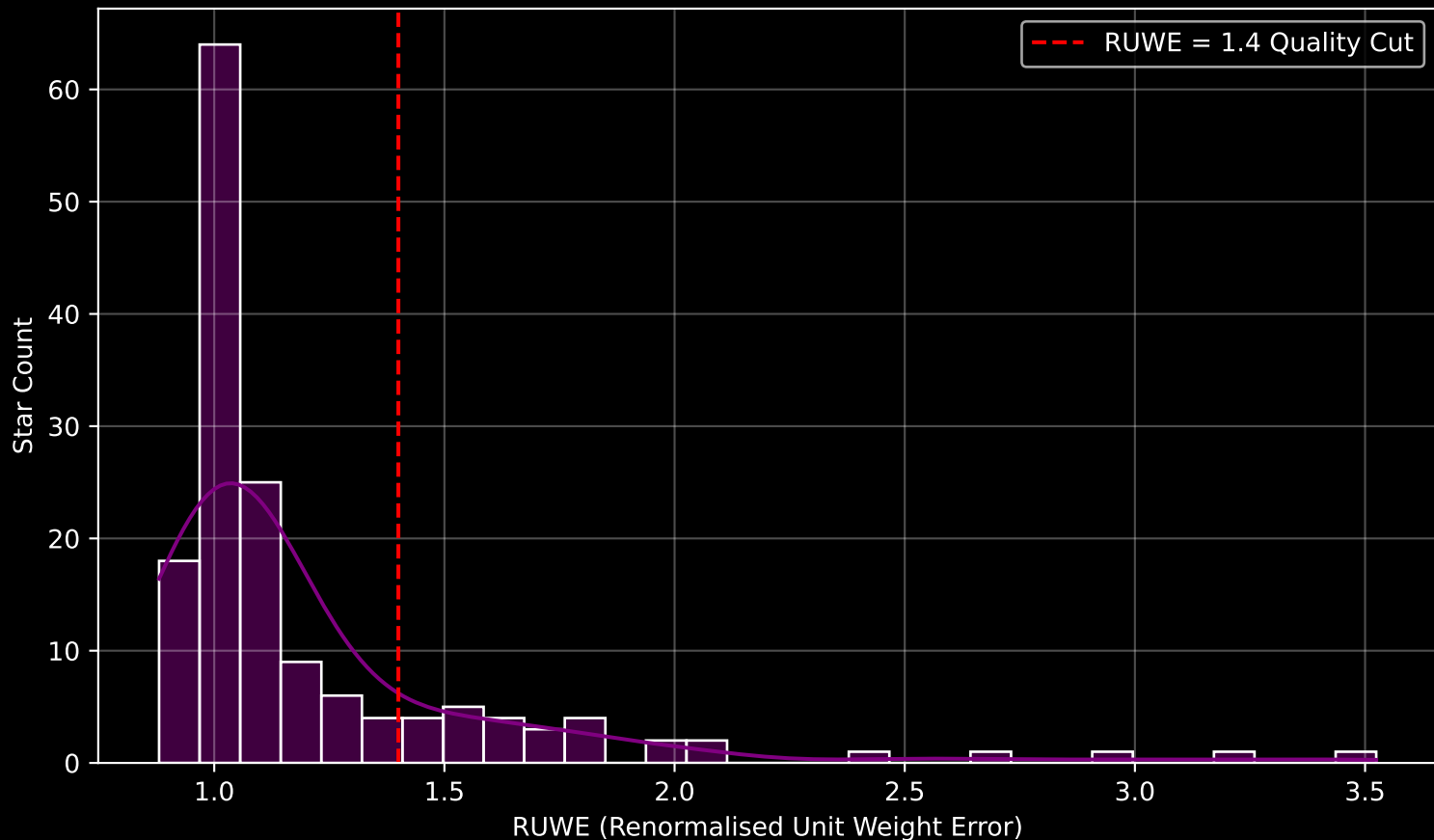
GAPOGEE DR17 Field [120-45] RUWE Distribution (n= 155)
